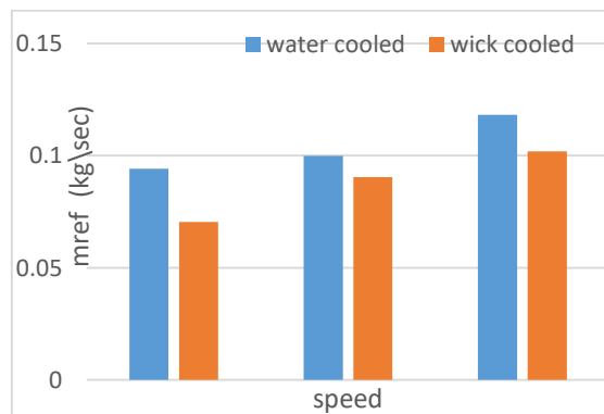
Fig 7: Comparison of Mass Flow Rate
