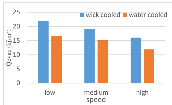
Fig 5: Comparison of Refrigeration Effect
